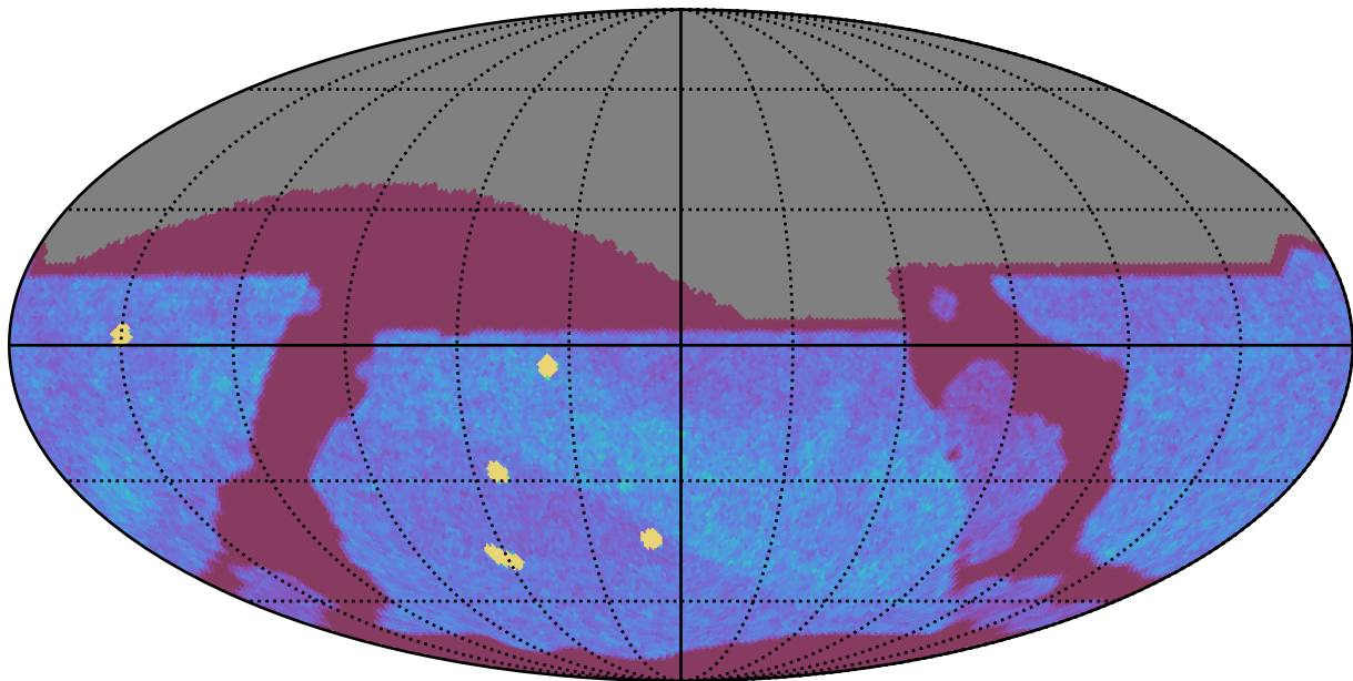
too_100_1v3.4_10yrs All sky z band: NVisits
