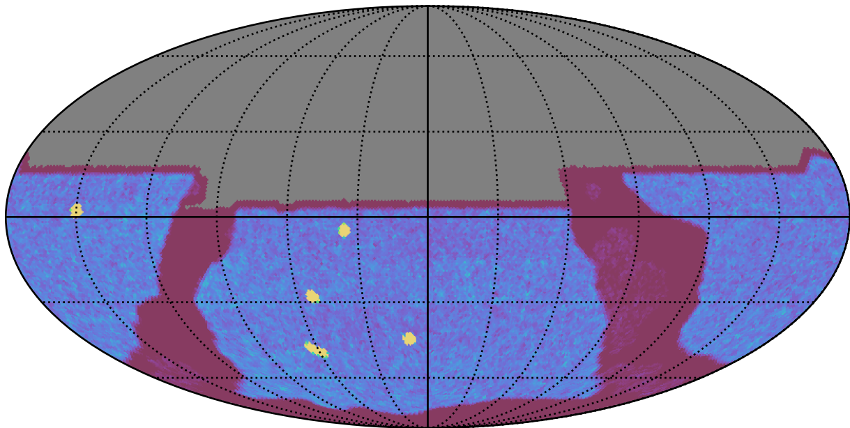
too_100_1v3.4_10yrs All sky y band: NVisits
