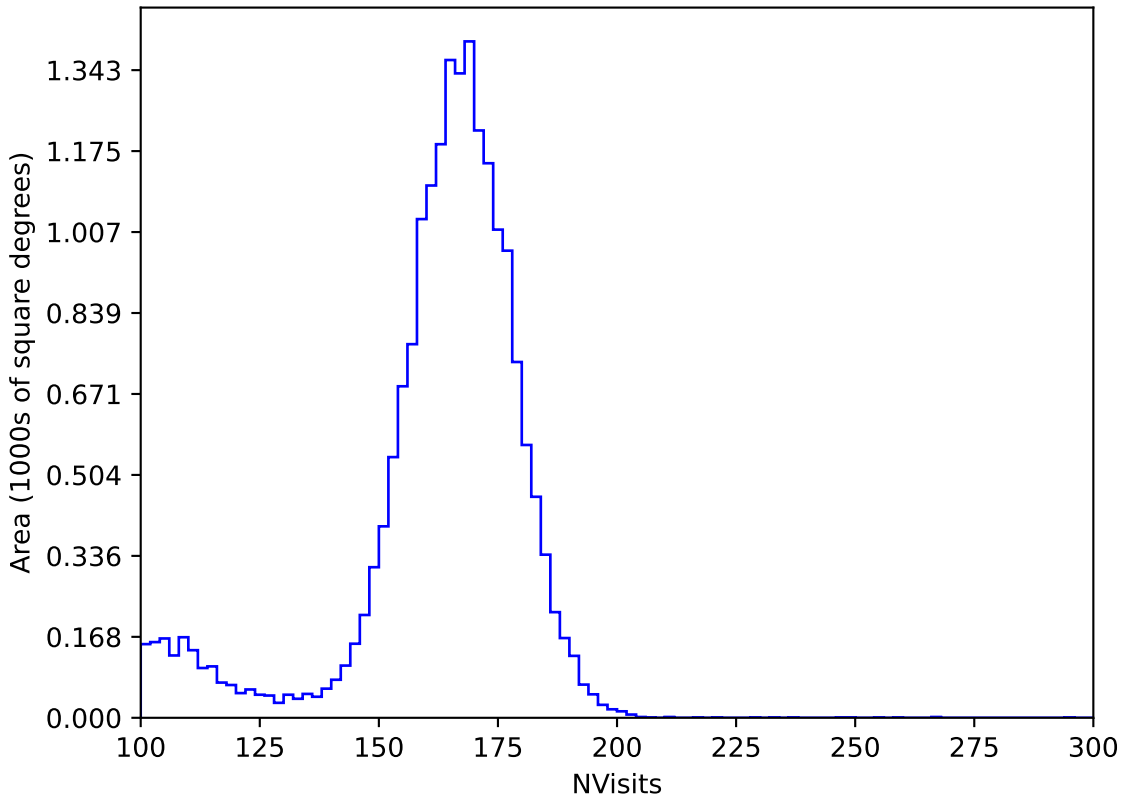
too_100_1v3.4_10yrs All sky y band: NVisits
