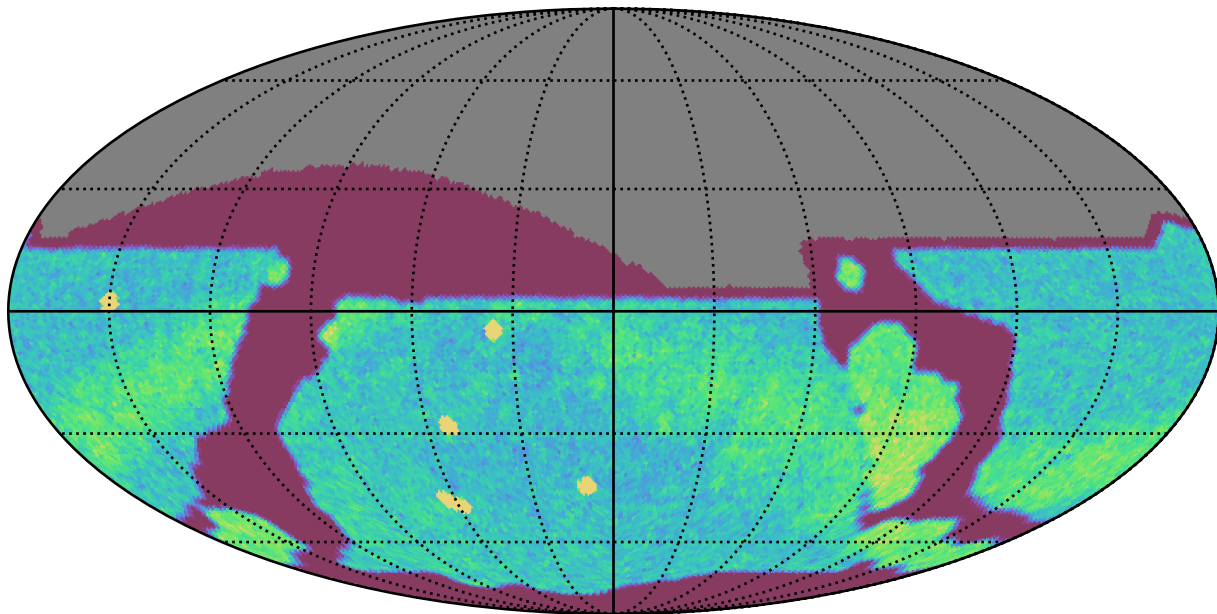
too_100_1v3.4_10yrs All sky r band: NVisits
