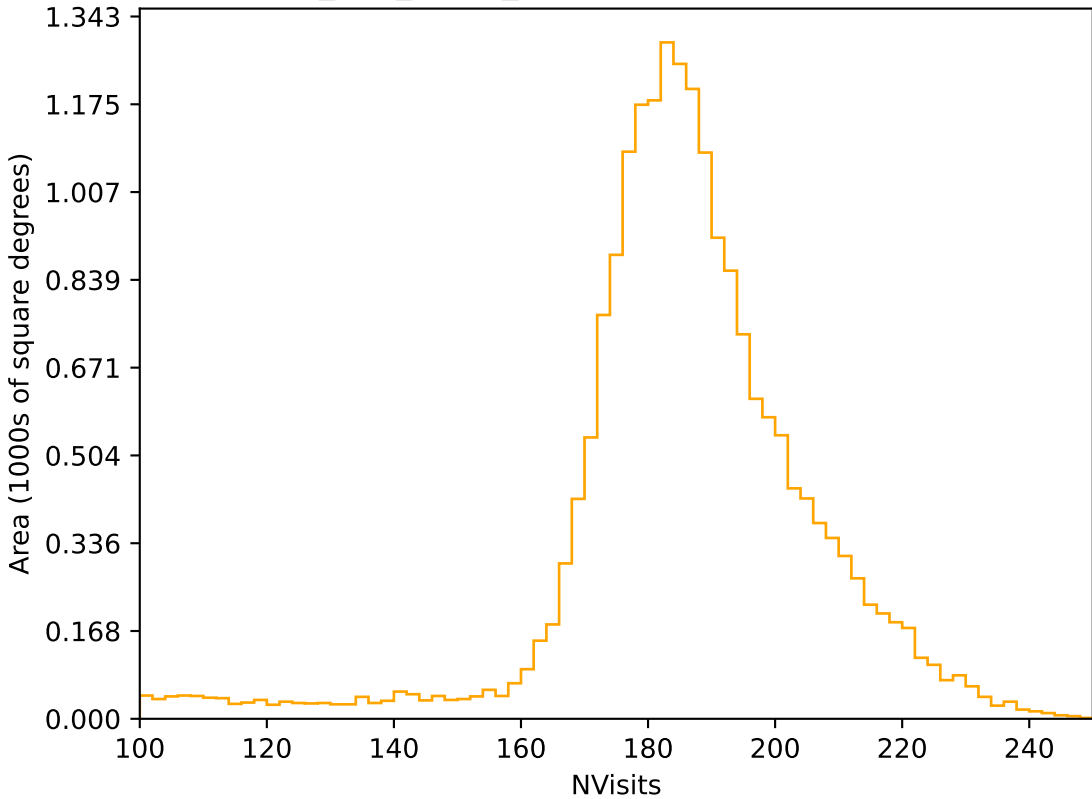
too_100_1v3.4_10yrs All sky r band: NVisits
