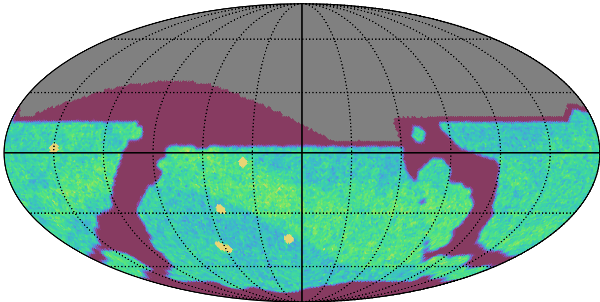
too_100_1v3.4_10yrs All sky i band: NVisits
