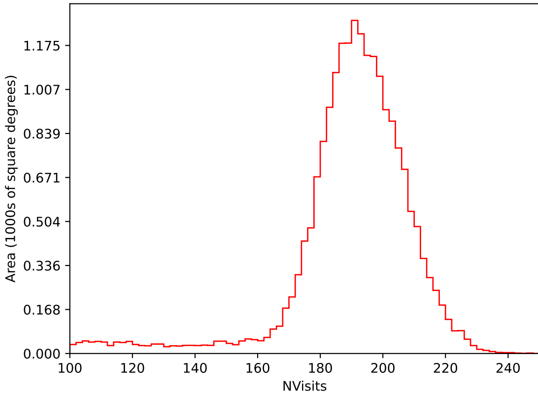
too_100_1v3.4_10yrs All sky i band: NVisits
