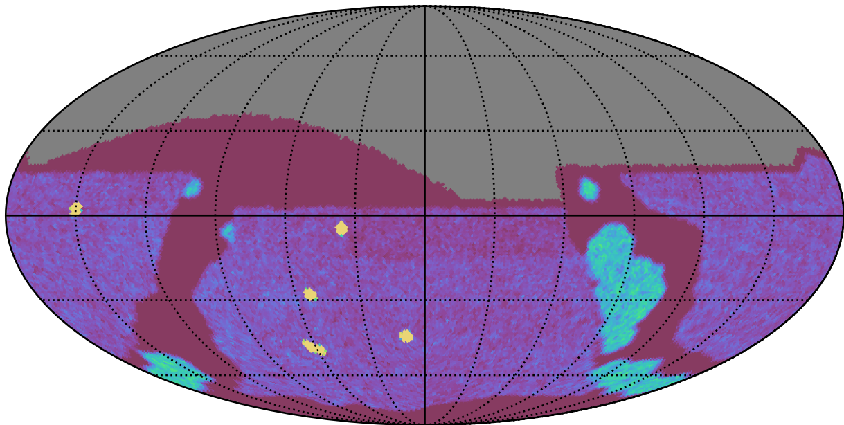
too_100_1v3.4_10yrs All sky g band: NVisits
