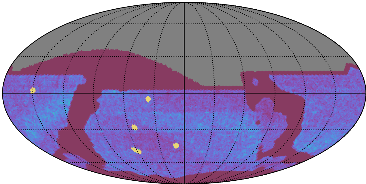
too_100_1v3.4_10yrs All sky all bands: NVisits
