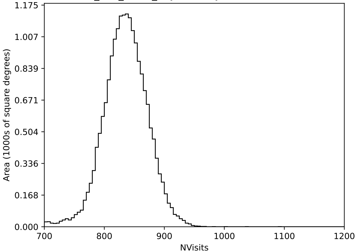
too_100_1v3.4_10yrs All sky all bands: NVisits
