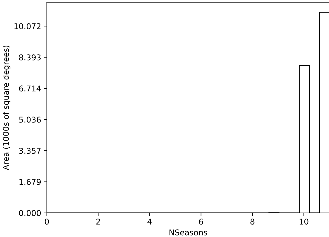
too_100_1v3.4_10yrs WFD all bands: NSeasons
