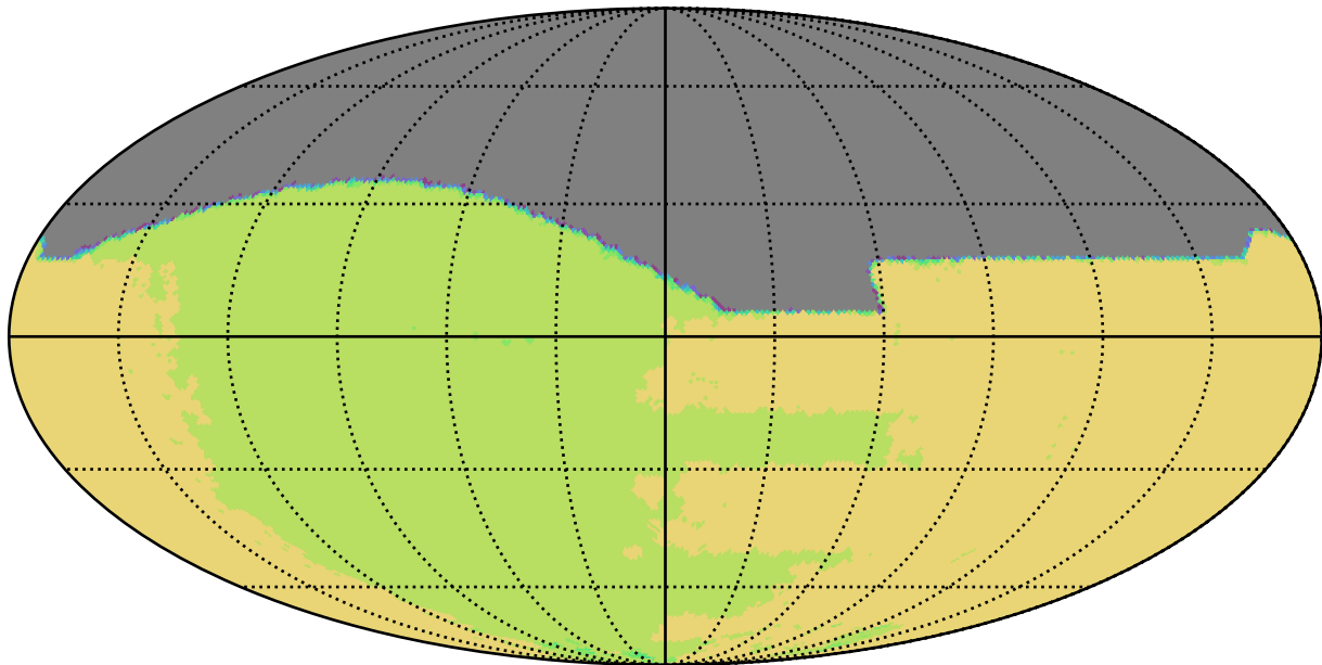
too_100_1v3.4_10yrs All sky all bands: NSeasons
