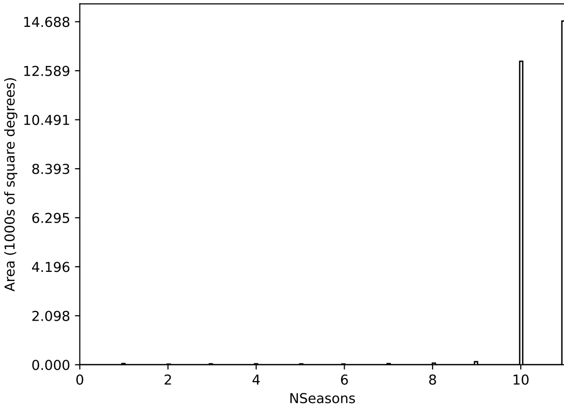
too_100_1v3.4_10yrs All sky all bands: NSeasons
