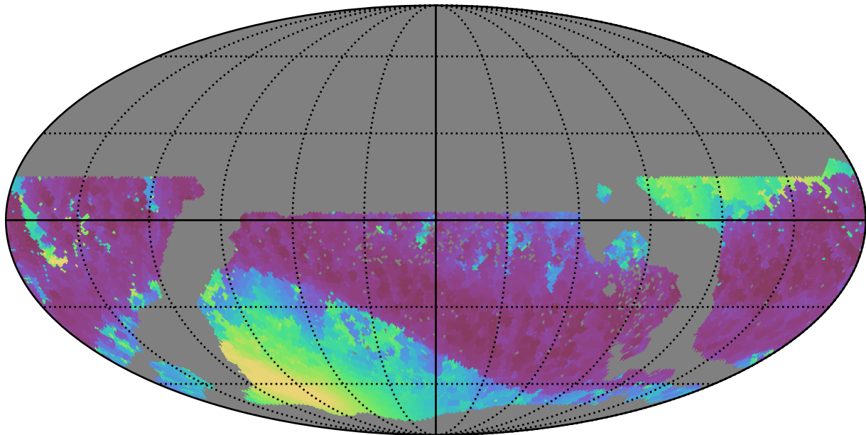
too_100_1v3.4_10yrs WFD z band: Min solarElong
