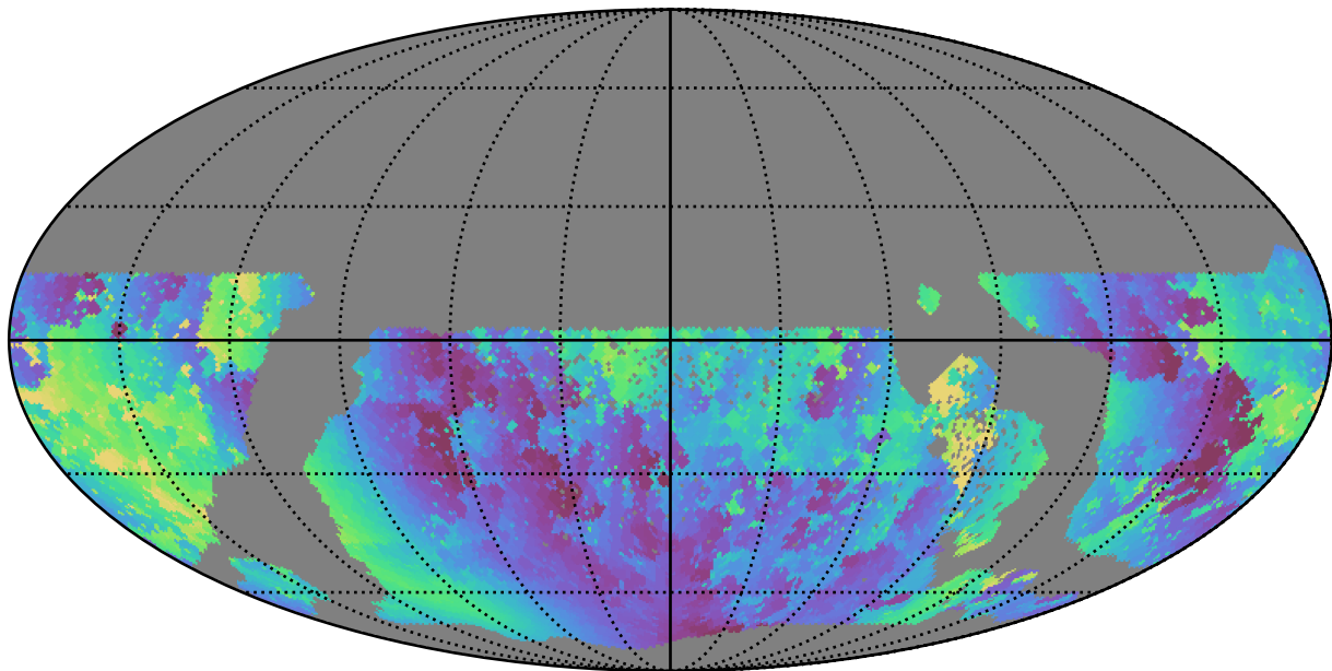
too_100_1v3.4_10yrs WFD u band: Min solarElong
