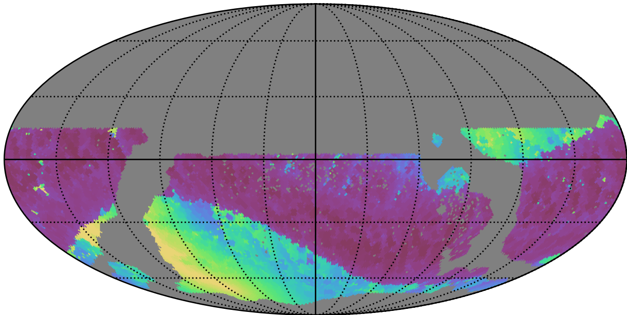
too_100_1v3.4_10yrs WFD i band: Min solarElong
