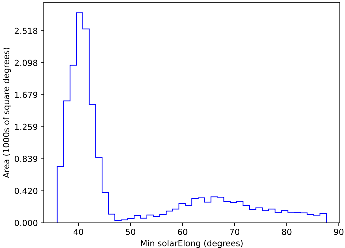
too_100_1v3.4_10yrs WFD i band: Min solarElong
