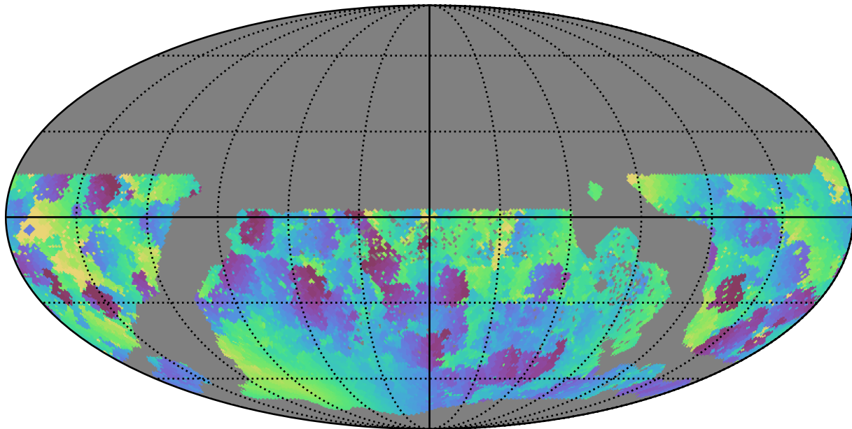
too_100_1v3.4_10yrs WFD g band: Min solarElong
