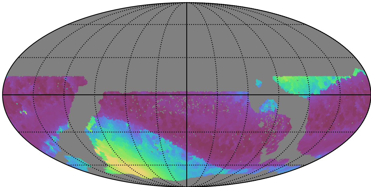
too_100_1v3.4_10yrs WFD all bands: Min solarElong
