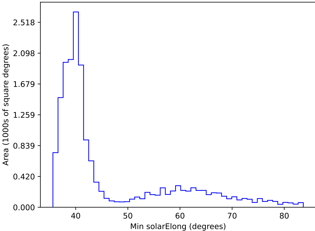
too_100_1v3.4_10yrs WFD all bands: Min solarElong
