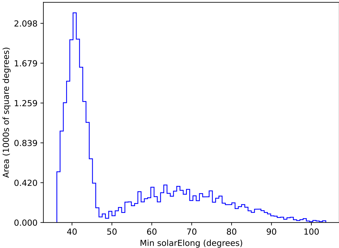
too_100_1v3.4_10yrs All sky z band: Min solarElong
