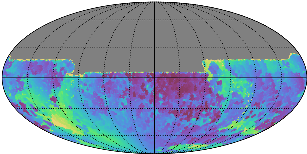
too_100_1v3.4_10yrs All sky y band: Min solarElong
