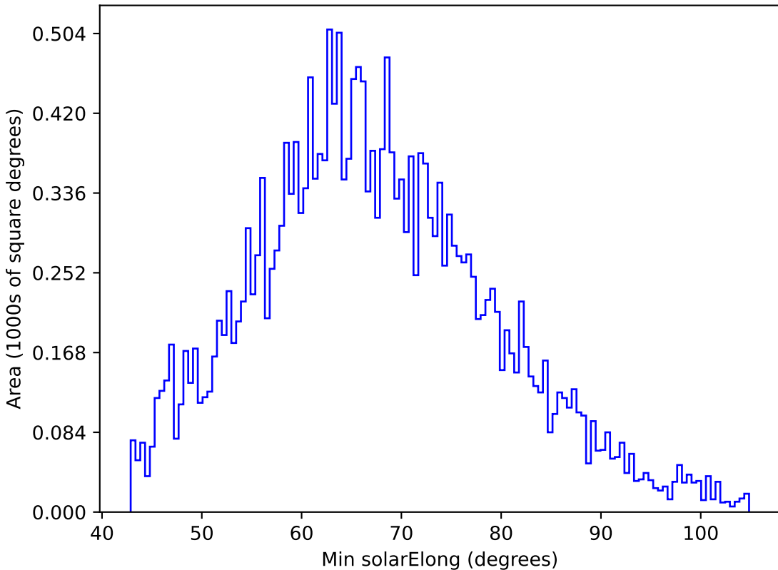
too_100_1v3.4_10yrs All sky y band: Min solarElong
