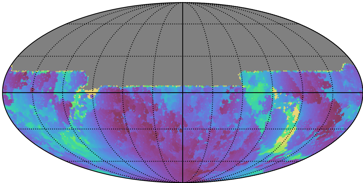
too_100_1v3.4_10yrs All sky u band: Min solarElong
