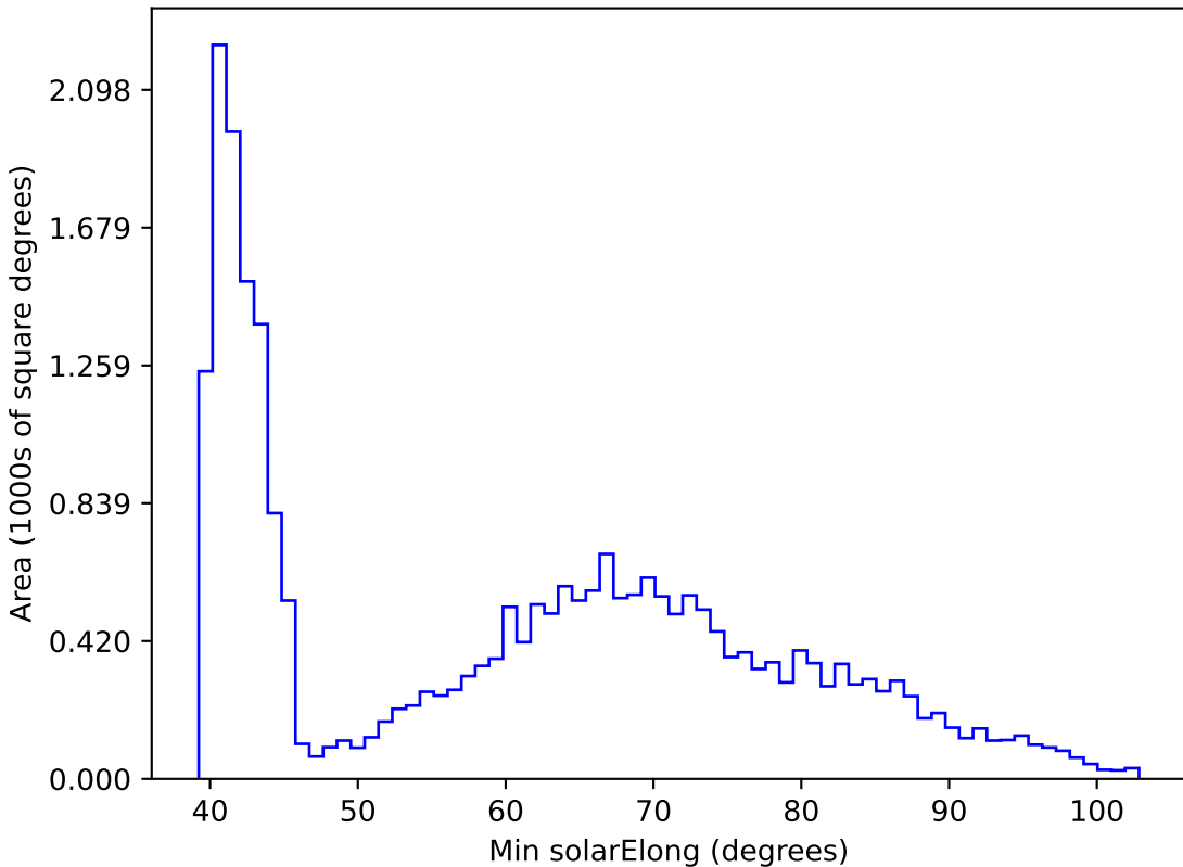
too_100_1v3.4_10yrs All sky r band: Min solarElong
