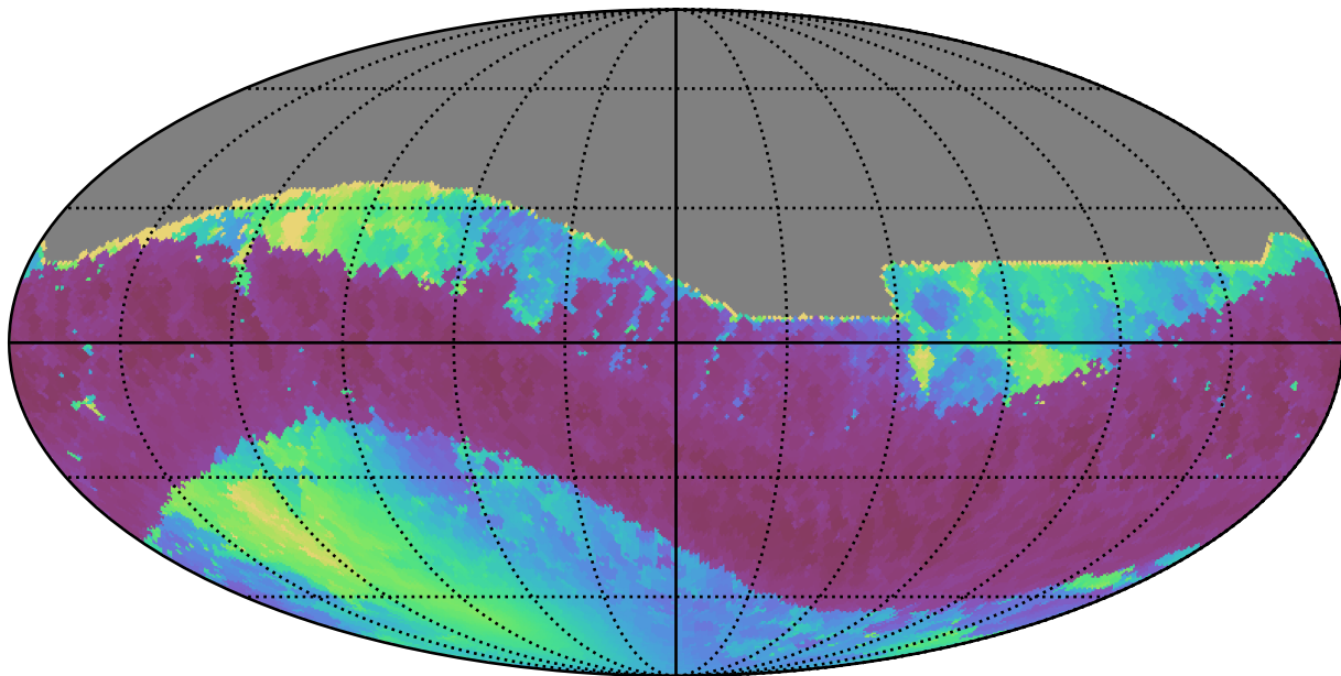
too_100_1v3.4_10yrs All sky i band: Min solarElong
