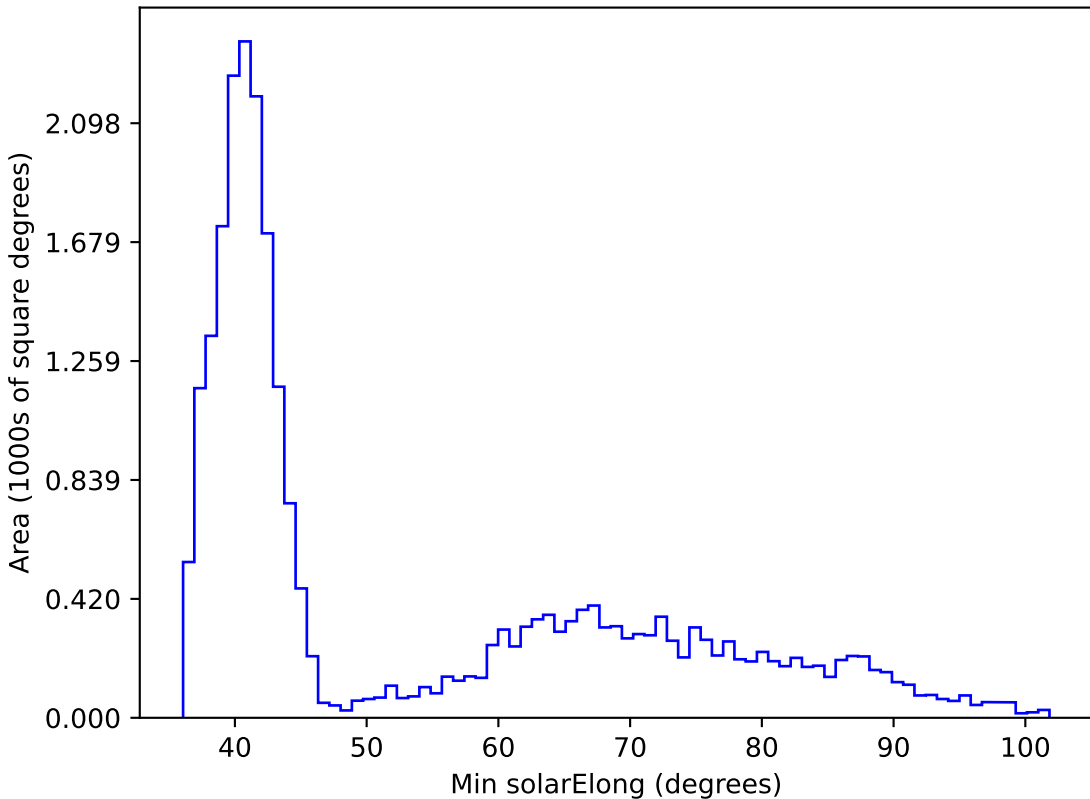
too_100_1v3.4_10yrs All sky i band: Min solarElong
