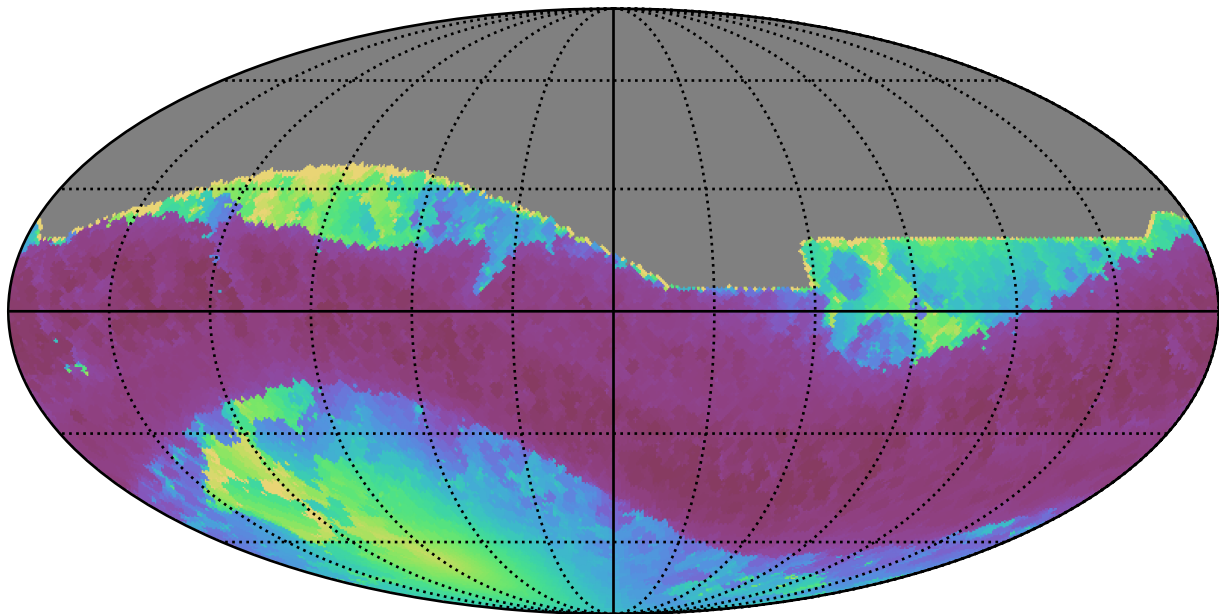
too_100_1v3.4_10yrs All sky all bands: Min solarElong
