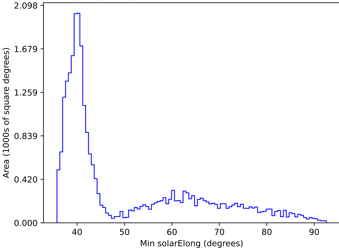
too_100_1v3.4_10yrs All sky all bands: Min solarElong
