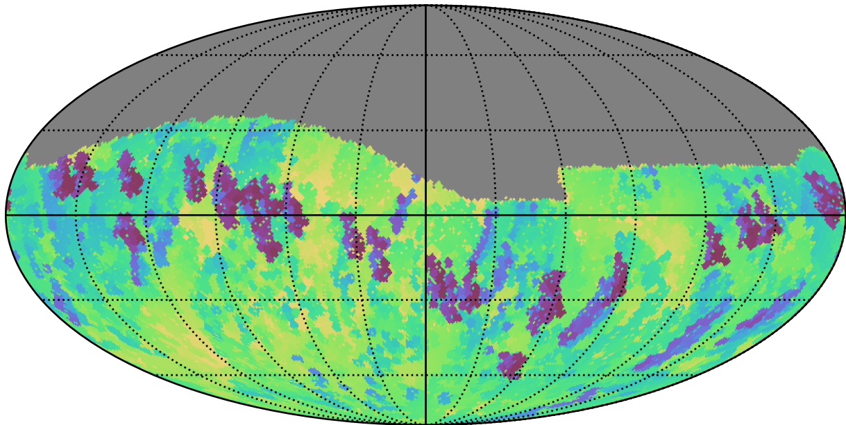
too_100_1v3.4_10yrs Yr 1 z band: Min skyBrightness
