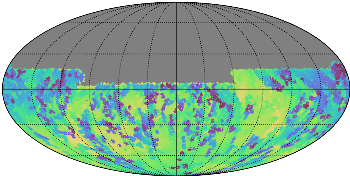
too_100_1v3.4_10yrs Yr 1 y band: Min skyBrightness
