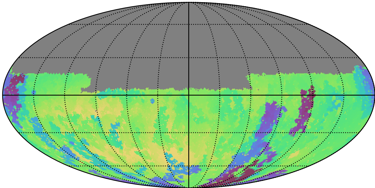
too_100_1v3.4_10yrs Yr 1 u band: Min skyBrightness
