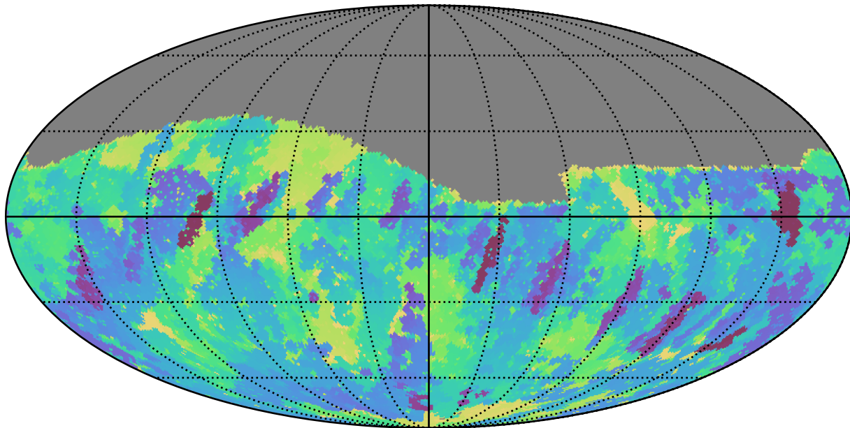
too_100_1v3.4_10yrs Yr 1 r band: Min skyBrightness
