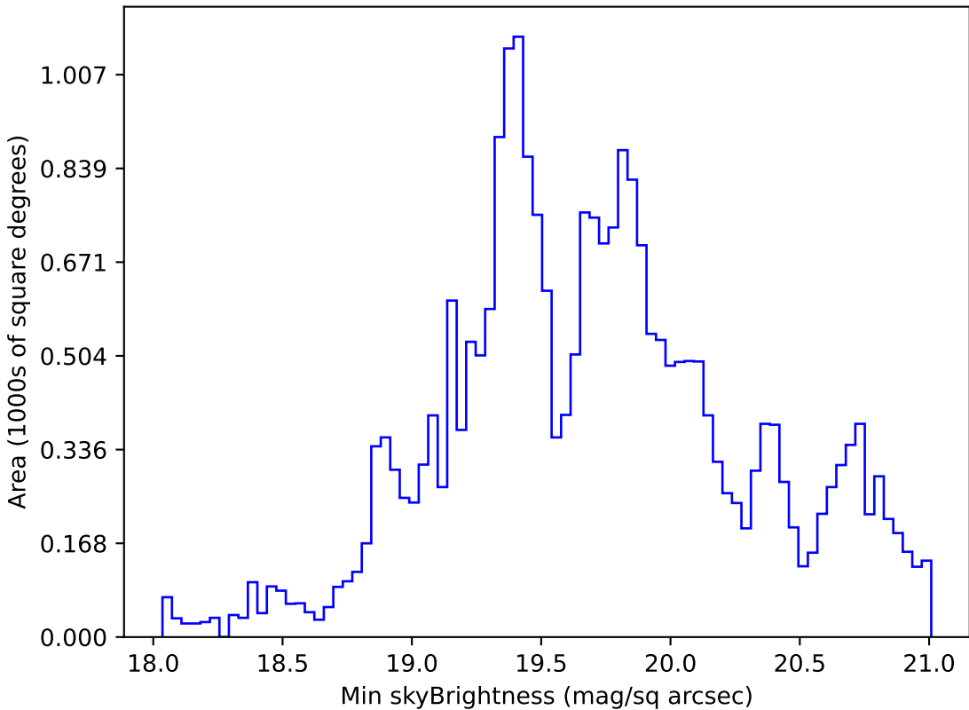
too_100_1v3.4_10yrs Yr 1 r band: Min skyBrightness
