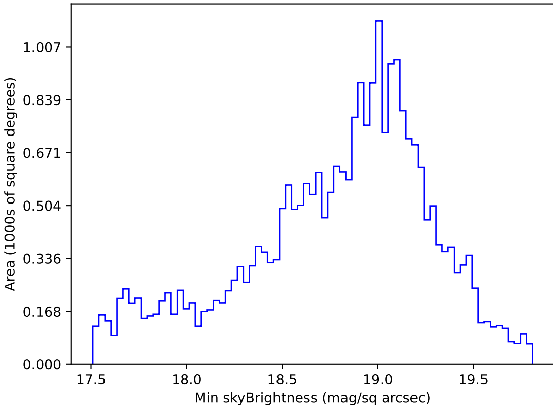
too_100_1v3.4_10yrs Yr 1 i band: Min skyBrightness
