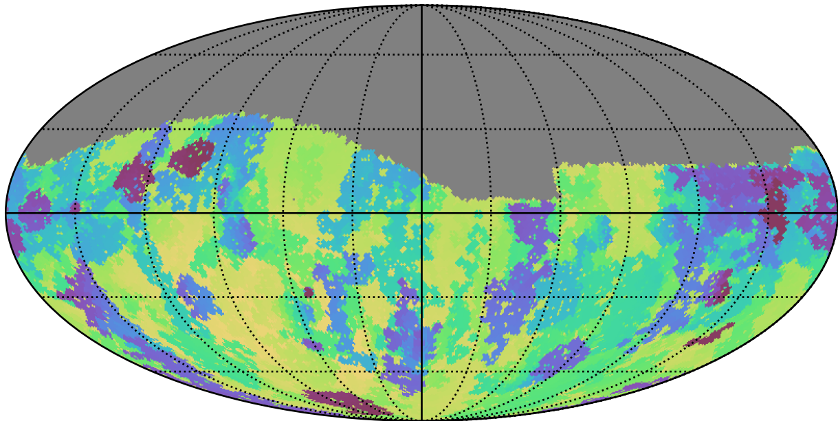
too_100_1v3.4_10yrs Yr 1 g band: Min skyBrightness
