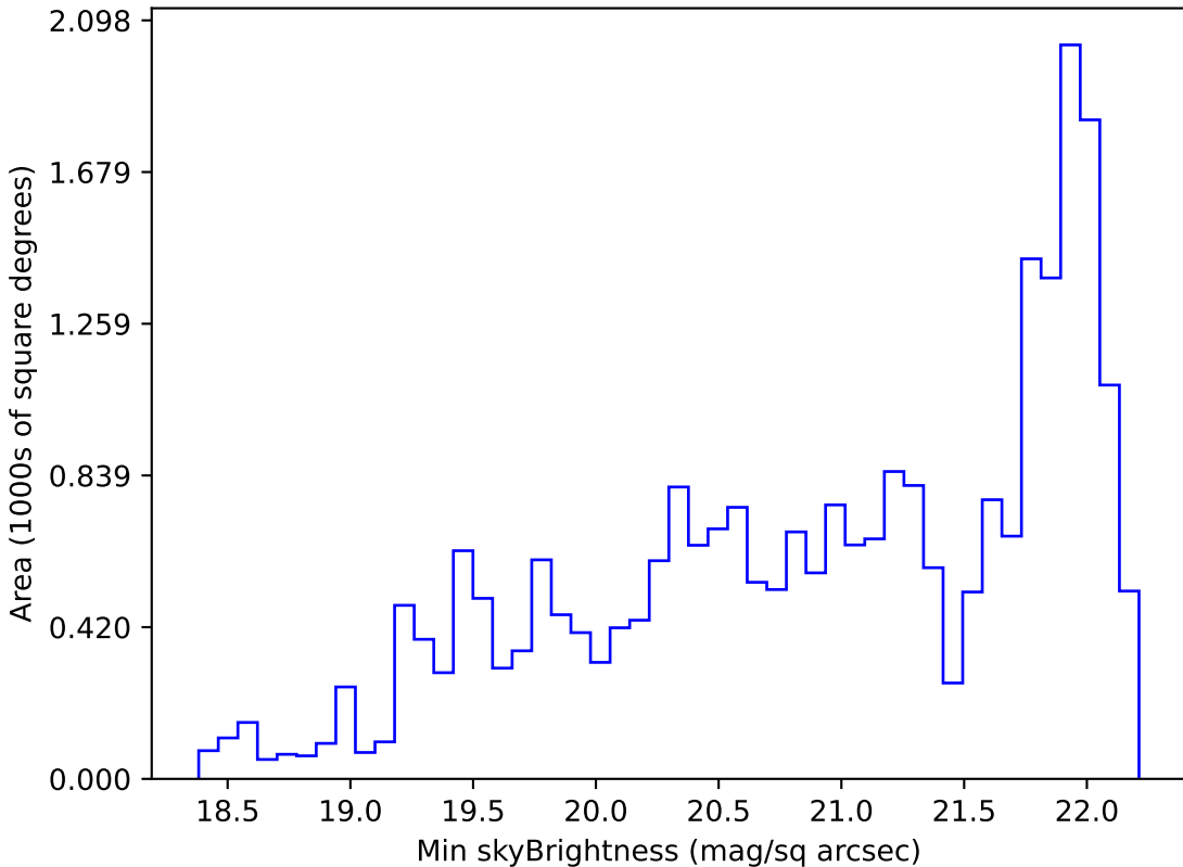
too_100_1v3.4_10yrs Yr 1 g band: Min skyBrightness
