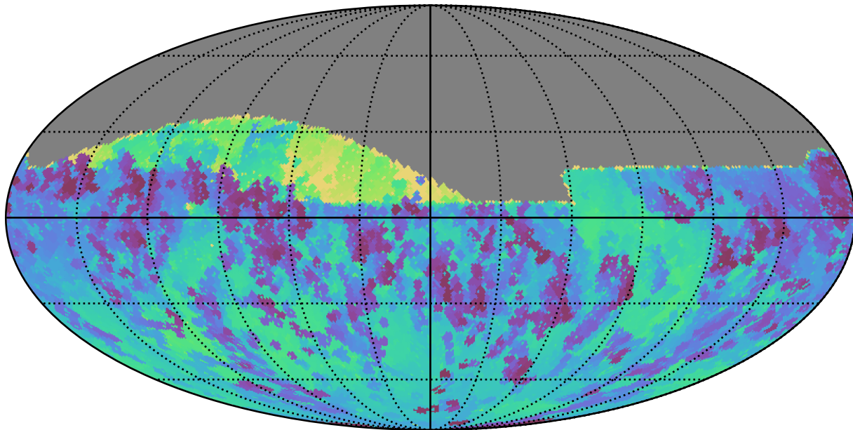
too_100_1v3.4_10yrs Yr 1 all bands: Min skyBrightness
