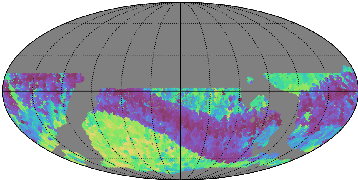
too_100_1v3.4_10yrs WFD z band: Min skyBrightness
