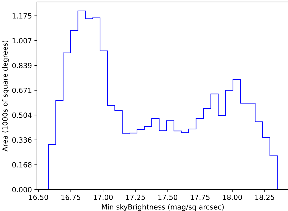
too_100_1v3.4_10yrs WFD z band: Min skyBrightness
