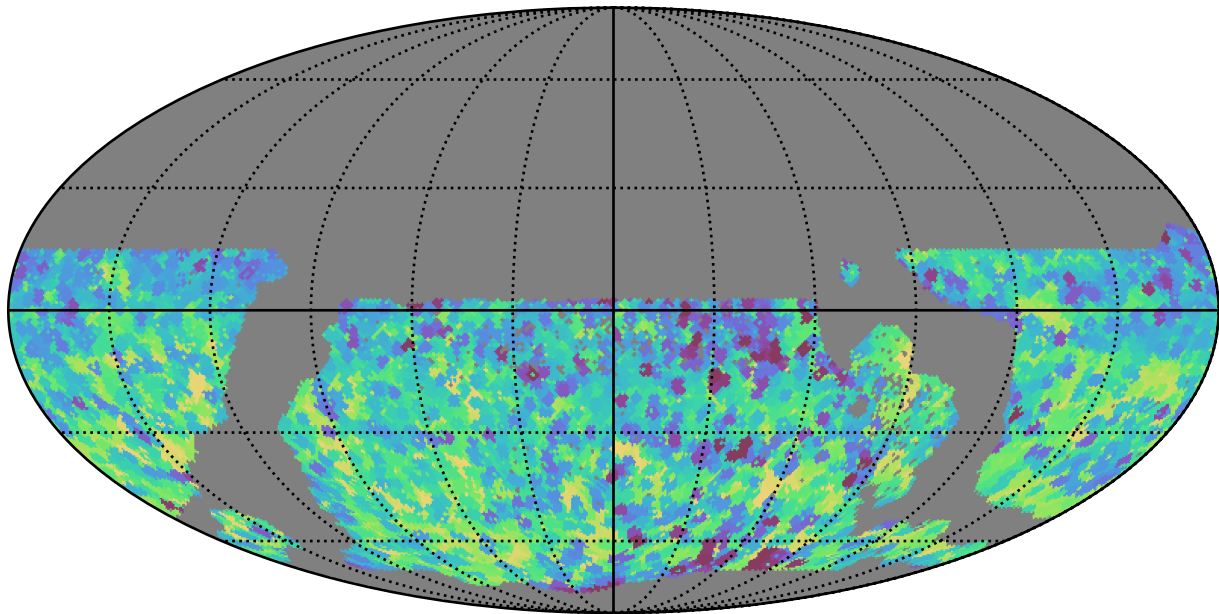
too_100_1v3.4_10yrs WFD y band: Min skyBrightness
