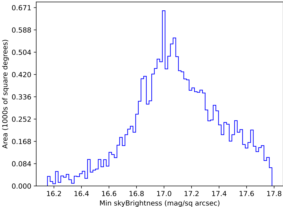
too_100_1v3.4_10yrs WFD y band: Min skyBrightness
