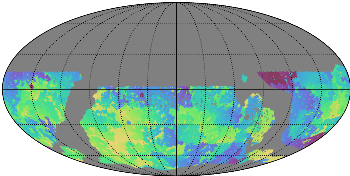
too_100_1v3.4_10yrs WFD u band: Min skyBrightness
