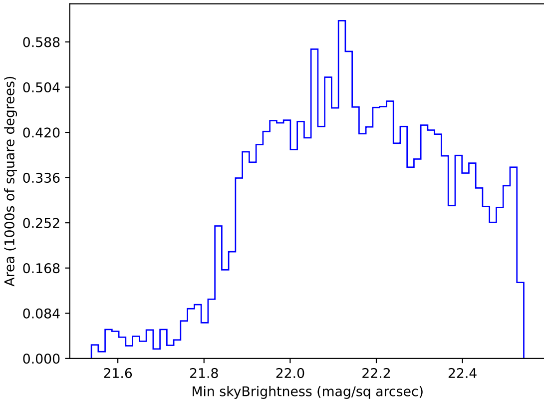
too_100_1v3.4_10yrs WFD u band: Min skyBrightness
