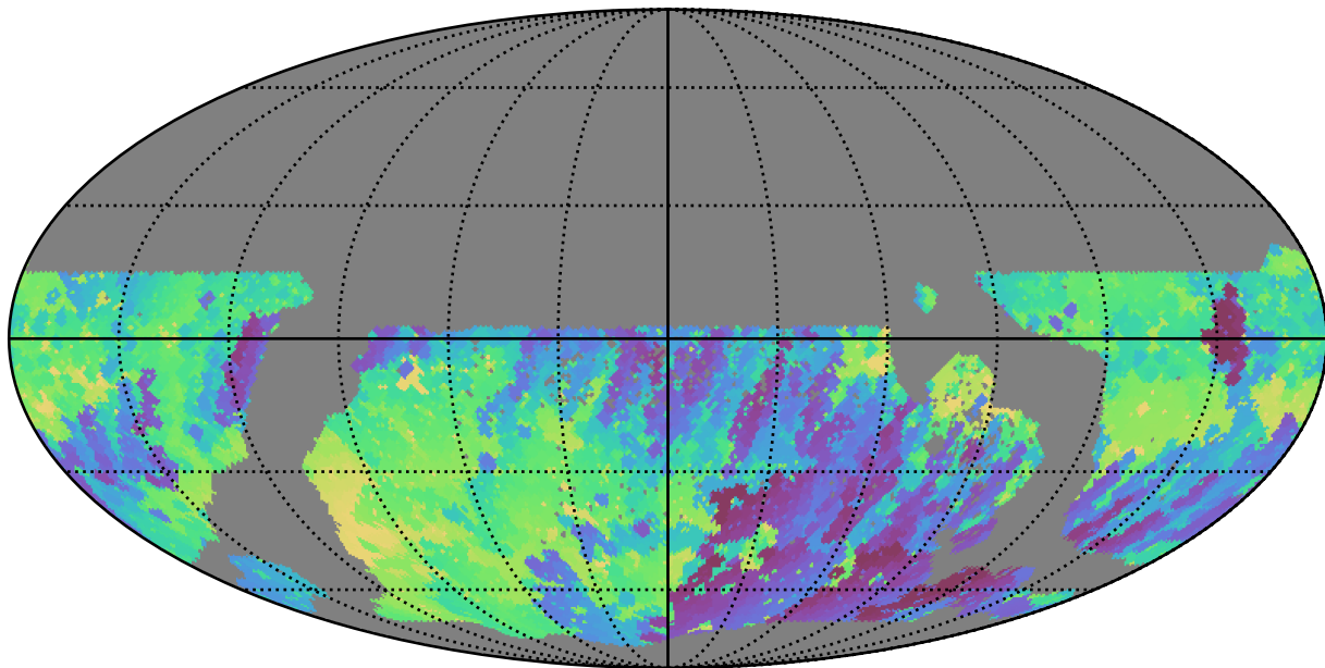
too_100_1v3.4_10yrs WFD r band: Min skyBrightness
