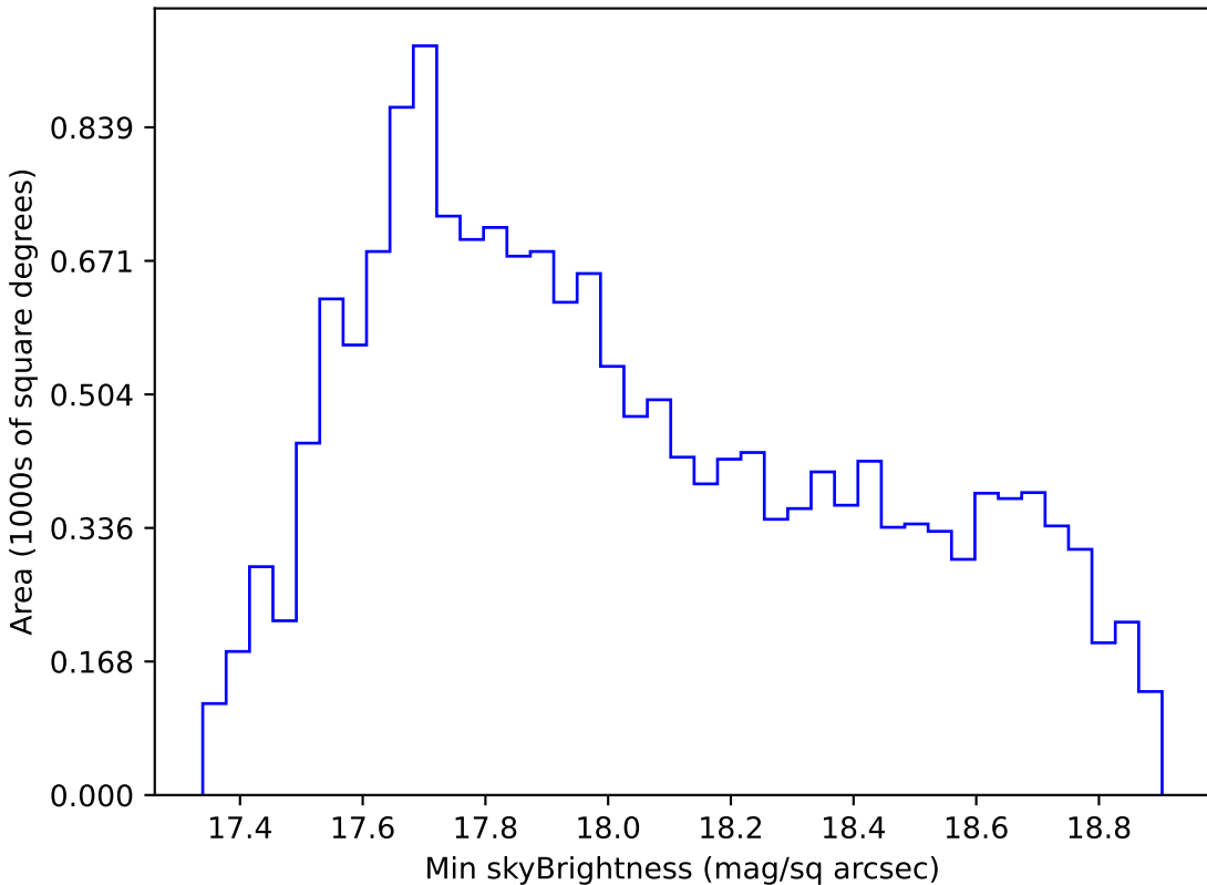
too_100_1v3.4_10yrs WFD i band: Min skyBrightness
