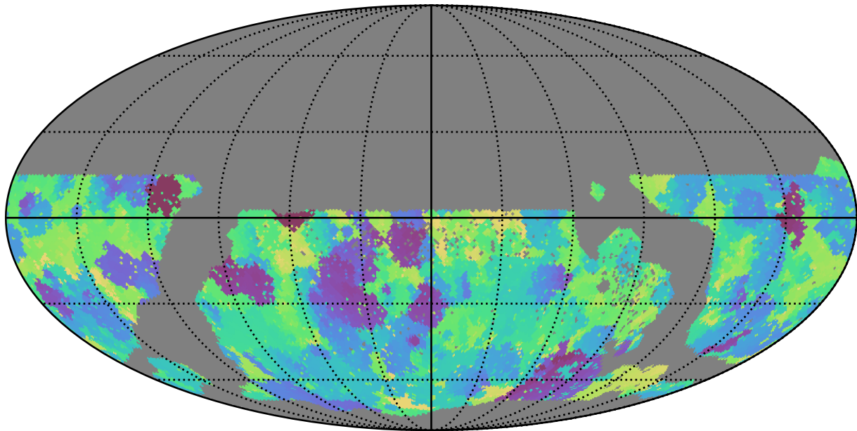
too_100_1v3.4_10yrs WFD g band: Min skyBrightness
