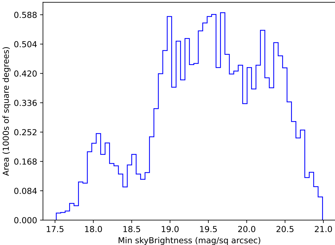
too_100_1v3.4_10yrs WFD g band: Min skyBrightness
