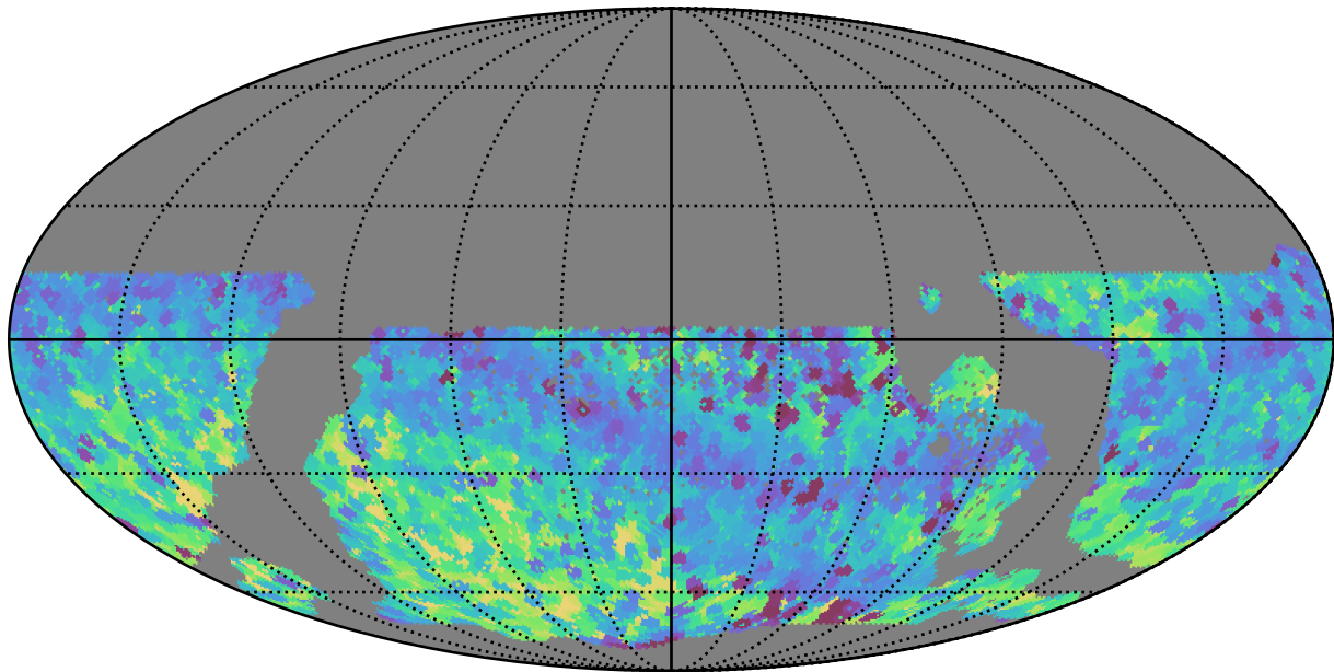
too_100_1v3.4_10yrs WFD all bands: Min skyBrightness
