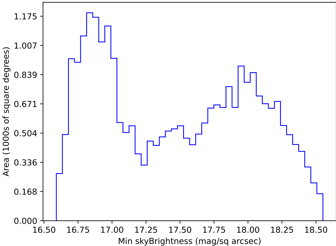
too_100_1v3.4_10yrs All sky z band: Min skyBrightness
